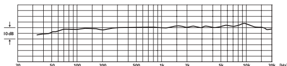
Frequenzgang Frequency response
